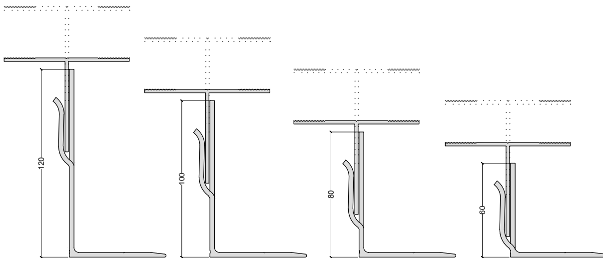
ADJUSTMENT 125 - 165mm
